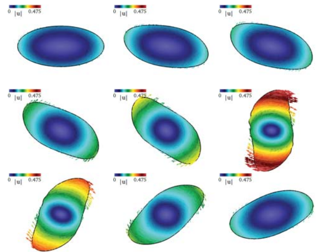
Fig. 5 Tumbling regime: Snapshots showing the dynamics of a membrane in simple shear flow (shape and velocity profile \Omega ) characterized by \Xi_{2d} = 0.65 , \mu^* = 10 , Re = 10^{-3} and \zeta = 1/2 at successive times t \in \{0, 1.25, 1.75, 2.5, 3, 4.25, 4.75, 5.51, 6.5\} , respectively
